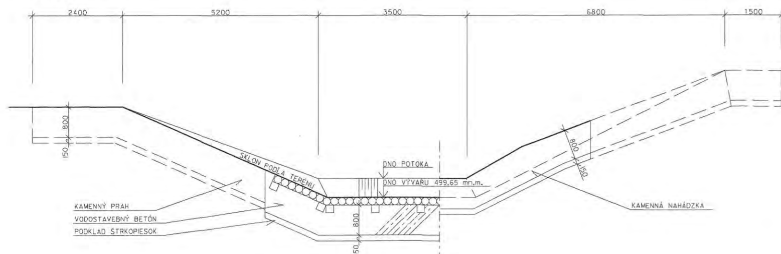
REZ III-III
