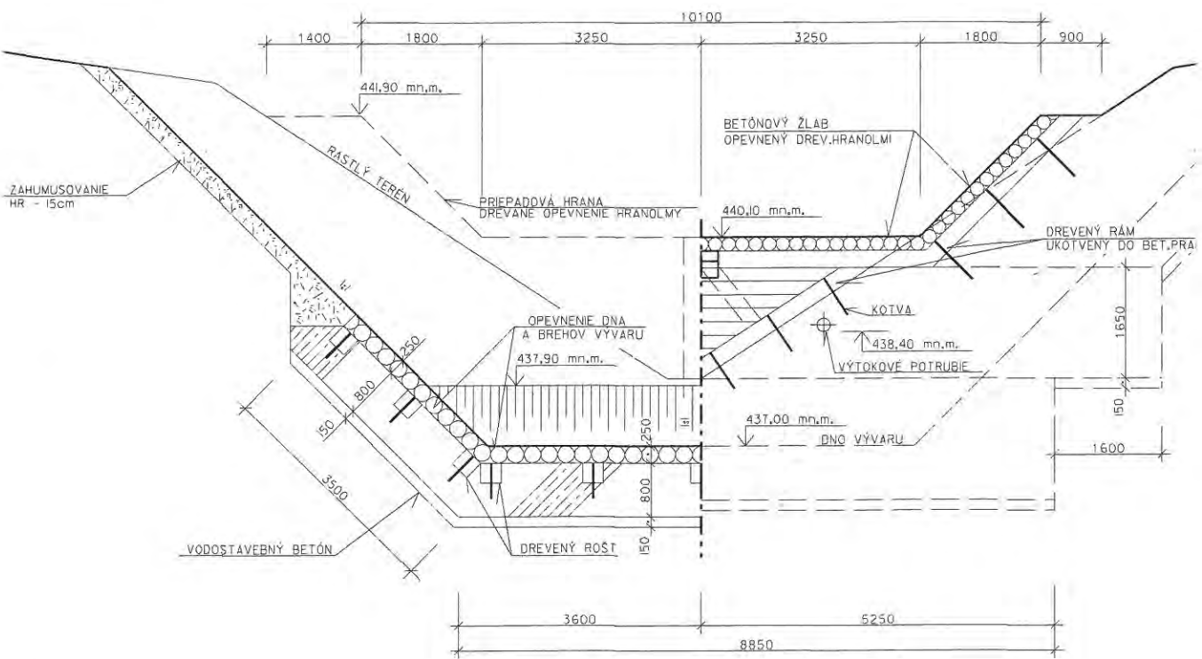
REZ IV-IV
