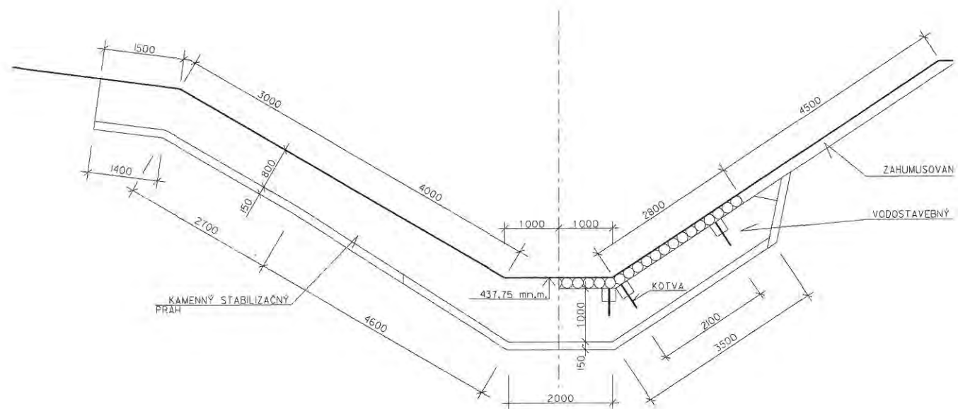
REZ IV-IV
